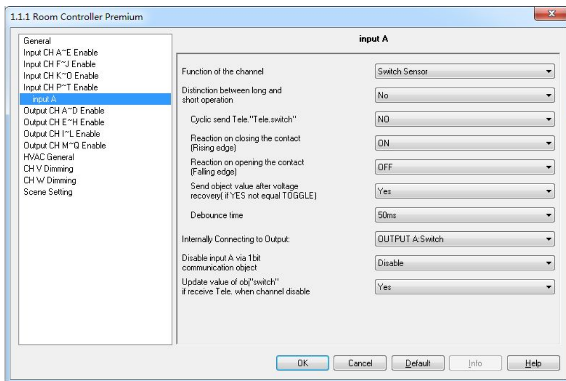
Fig. 5.8 Parameter window “Switch sensor” (No distinction long/short operation)
