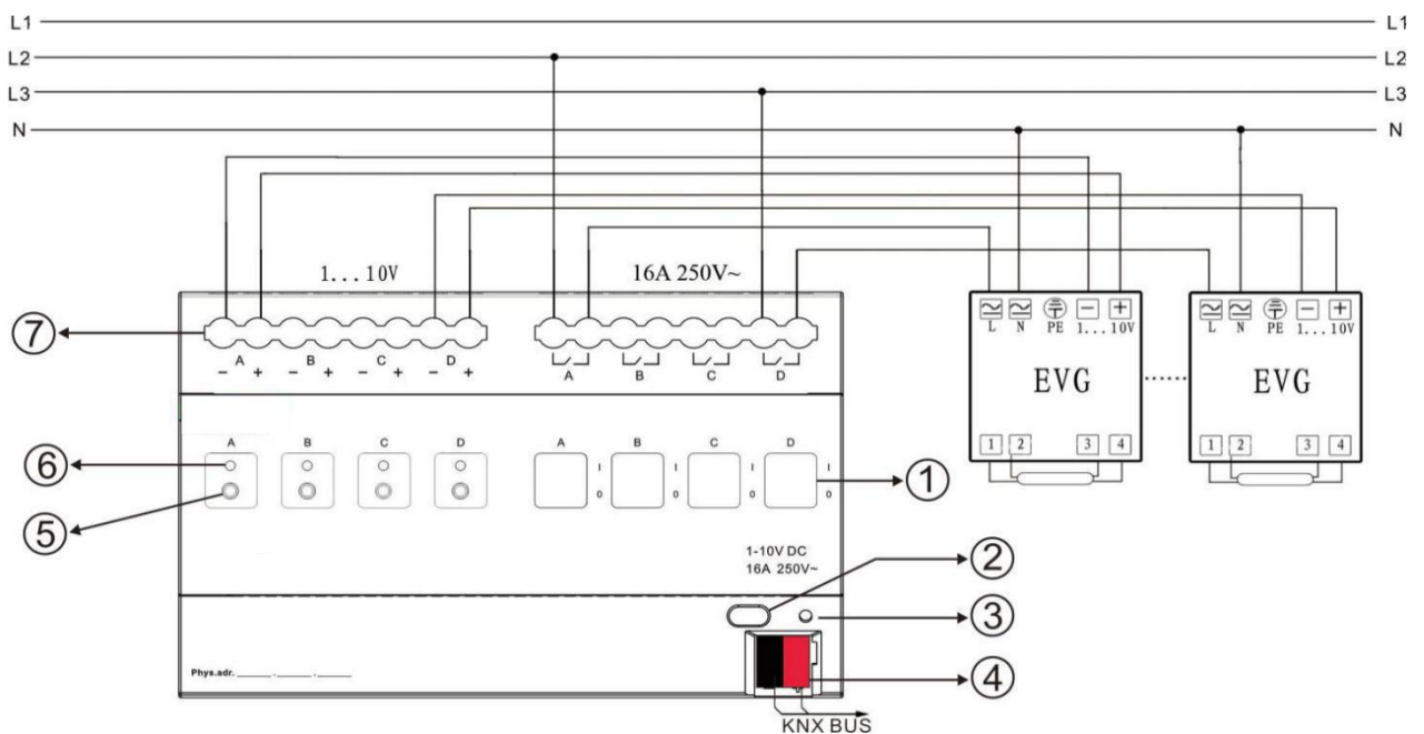
Connection Diagram:
