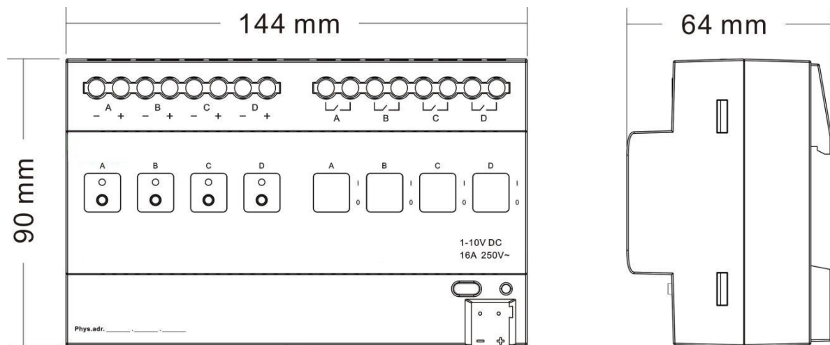
Dimension drawing:
